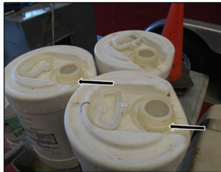
Breaks in lid ring seal as an indication that the cap has been potentially opened.
